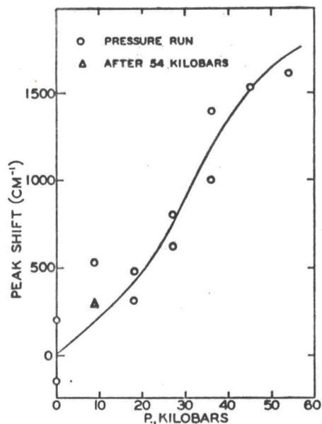
FIG. 12. Shift of dimer absorption peak at 21,700 \text{ cm}^{-1} vs pressure—acridine yellow in boric acid— 1.8 \times 10^{-4} \text{ g/g} .
